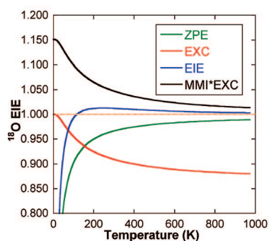
FIGURE 2. Calculated 18 O EIEs for formation of a Cu( \eta^1 -O 2 )TMG 3 Tren. 27
